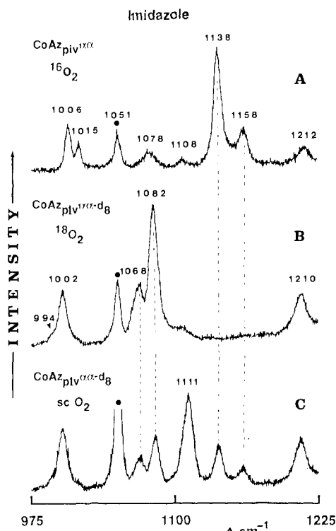
Figure 2. Resonance Raman spectra of O_2 adducts of CoAz_{piv}^{\alpha\alpha} complex with imidazole. Conditions as in text. The 1051\text{-cm}^{-1} line ( \bullet ) is due to C^2H_2Cl_2 .
