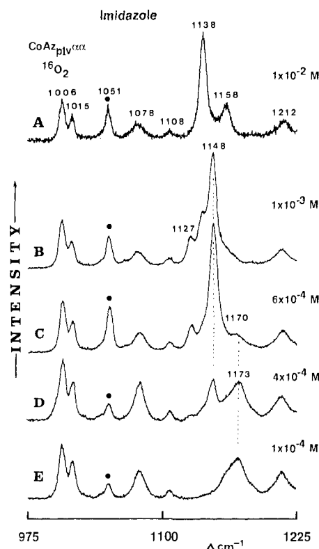
Figure 7. Resonance Raman spectra of the ^{16}\text{O}_2 adduct of \text{CoAz}_{\text{piv}}^{\alpha\alpha} complex with imidazole. Temperature \sim 185 K; imidazole concentrations estimated as described in text.
