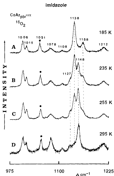
Figure 6. Resonance Raman spectra of the ^{16}\text{O}_2 adduct of \text{CoAz}_{\text{piv}}^{\alpha\alpha} complex with imidazole. Imidazole concentration between 1 \times 10^{-3} and 1 \times 10^{-2} M. Temperatures measured as described in text.
