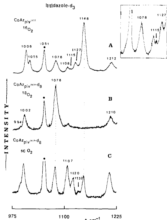
Figure 5. Resonance Raman spectra of O_2 adducts of CoAz_{piv}\alpha complex with imidazole- d_3 . See Figure 2 caption.
